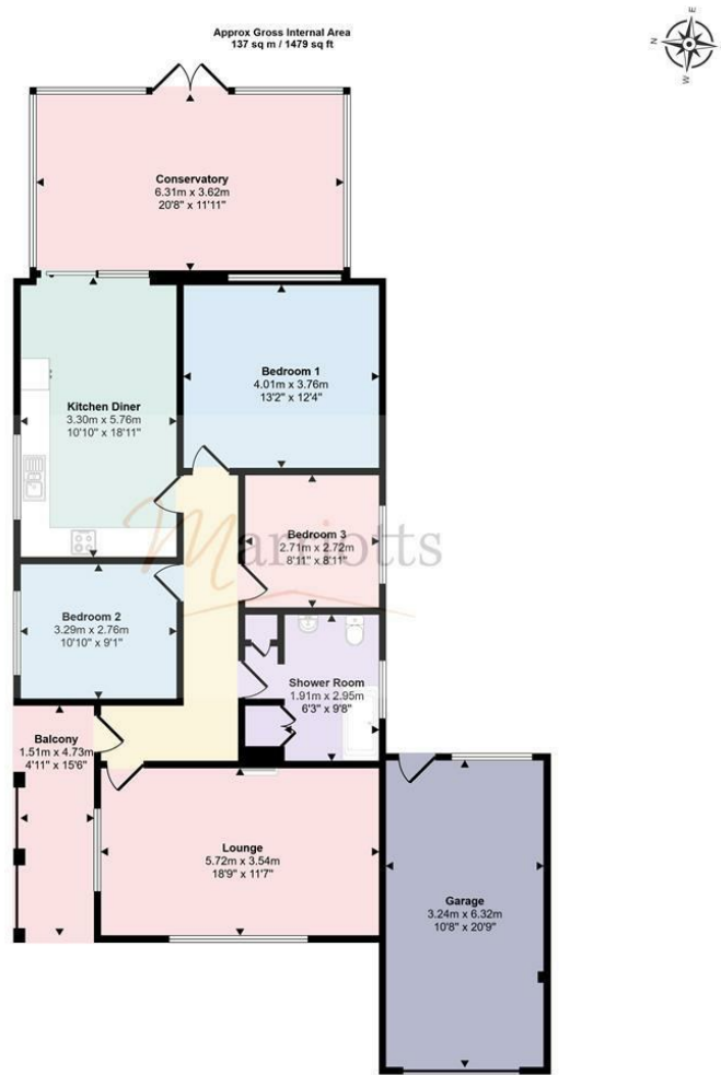
Floorplan
